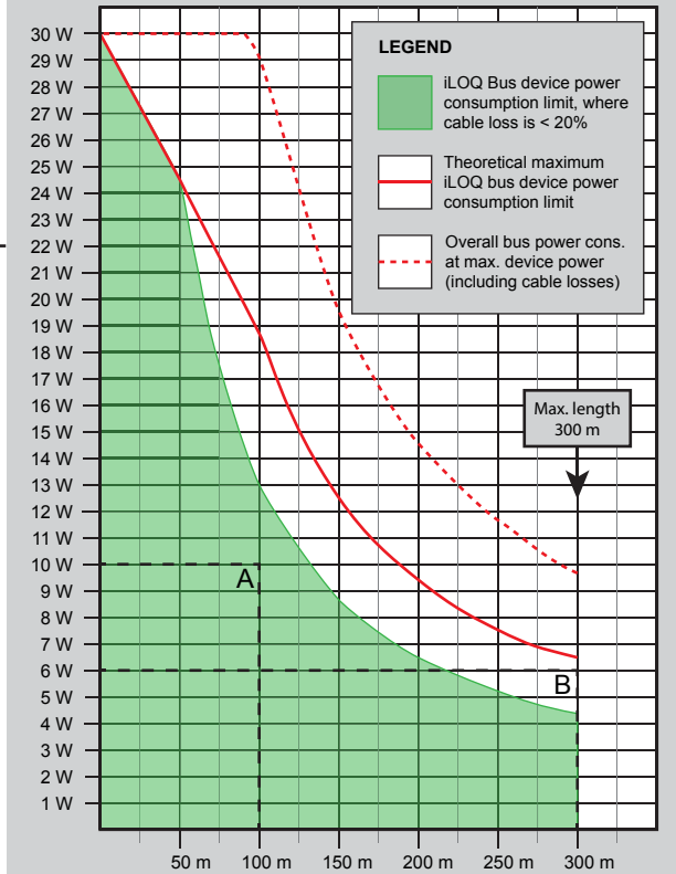
Graph 2. Maximum cumulative iLOQ bus device power and overall branch power consumption in relation to cable length
